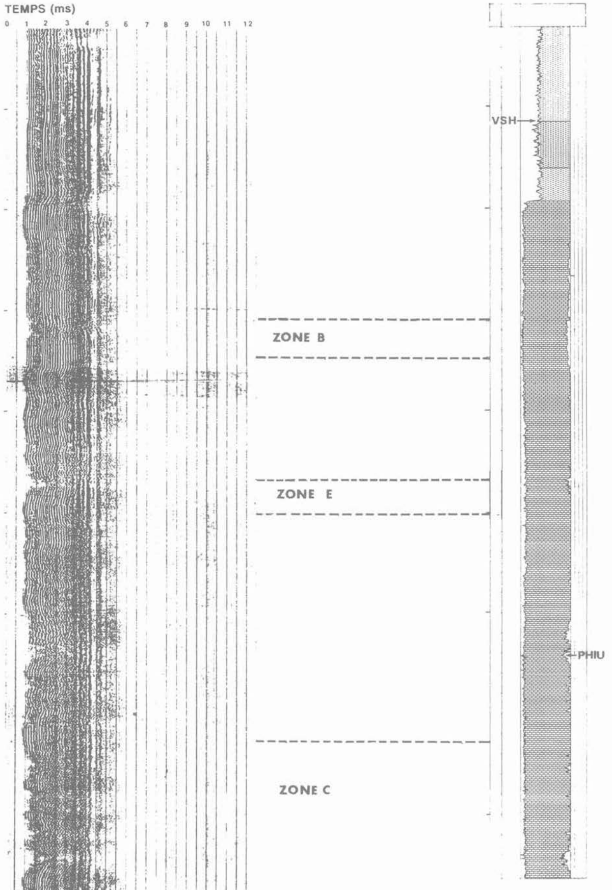
Fig. 13. — Iso-offset section and lithology from EVA for Gaviota 6.
