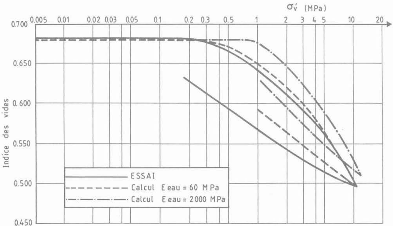
Fig. 7. — Gault inférieur. Essai œdométrique. Fig. 7. — Lower Gault - Compressibility tests - Comparison between model prediction and tests results.
