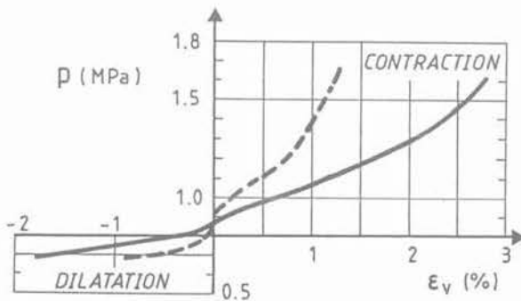
Fig. 5b. — Lower Gault - drained triaxial tests - Comparison between model prediction and tests results.
