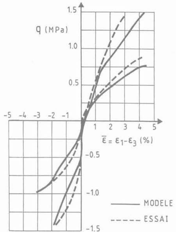
Fig. 6a. — Lower Gault - Undrained triaxial tests - Comparison between model prediction and tests results.
