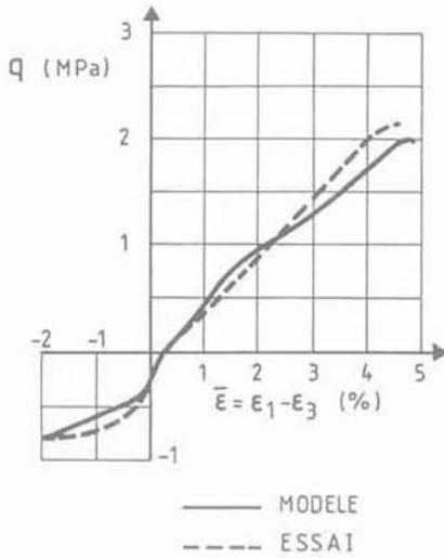
Fig. 5a. — Lower Gault - drained triaxial tests - Comparison between model prediction and tests results.
