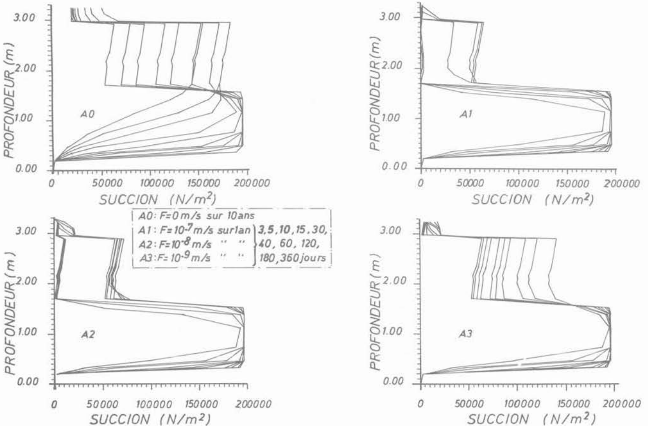
Fig. 5. — Simulations A Profils de succion. Fig. 5. — Simulations A Curves of suction.
