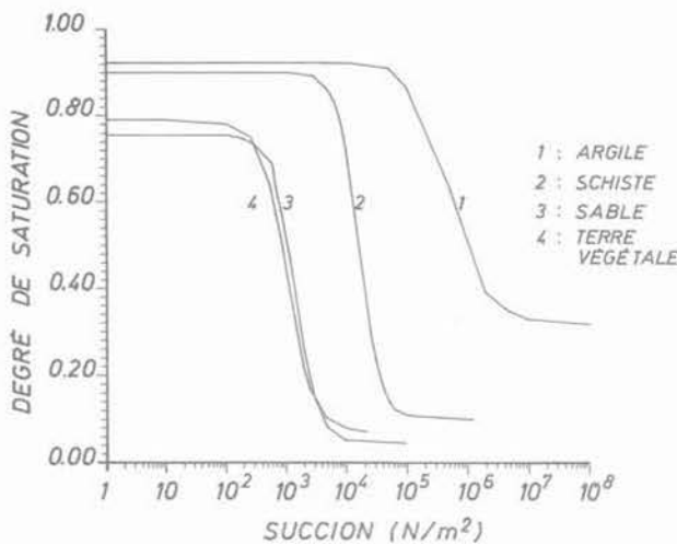
Fig. 2. — Courbes succion-degré de saturation. Fig. 2. — Curves suction-degree of saturation.
