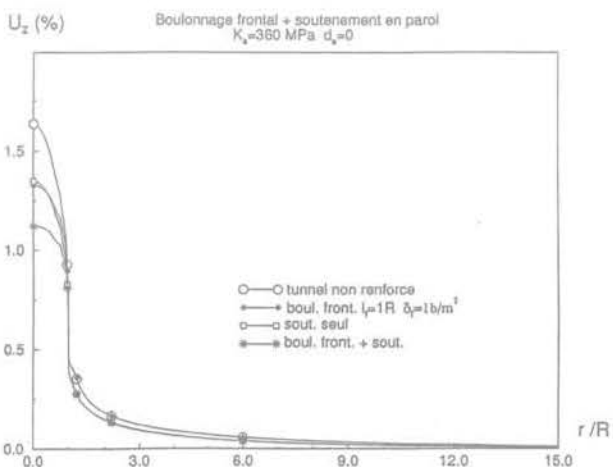
FIG.14 Influence du boulonnage frontal sur les convergences du tunnel soutenu. Influence of the facing bolts on the convergence of a tunnel with lining.
