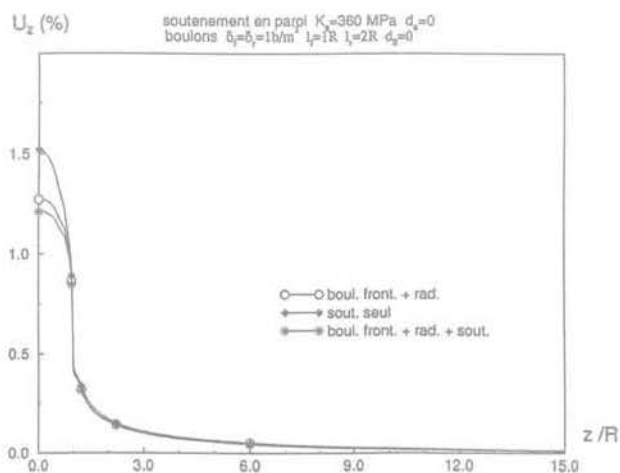
FIG.17 Association des deux modes de boulonnage au soutènement. Radial and facing bolts associated with lining.
