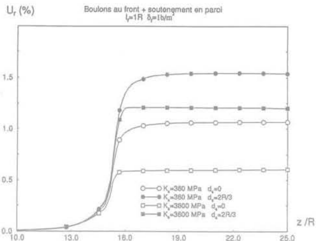
FIG.16 Influence de K_s et d_s . Influence of K_s and d_s .
