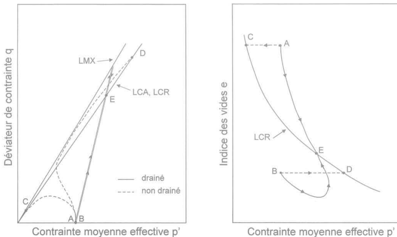
FIG. 12 Chemins drainés et non drainés dans les plans (q, p') et (e, p') . Drained and undrained effective stress paths in the (q, p') and (e, p') planes.
